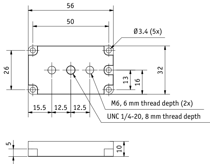
Figure 23: Tripod dimensions
