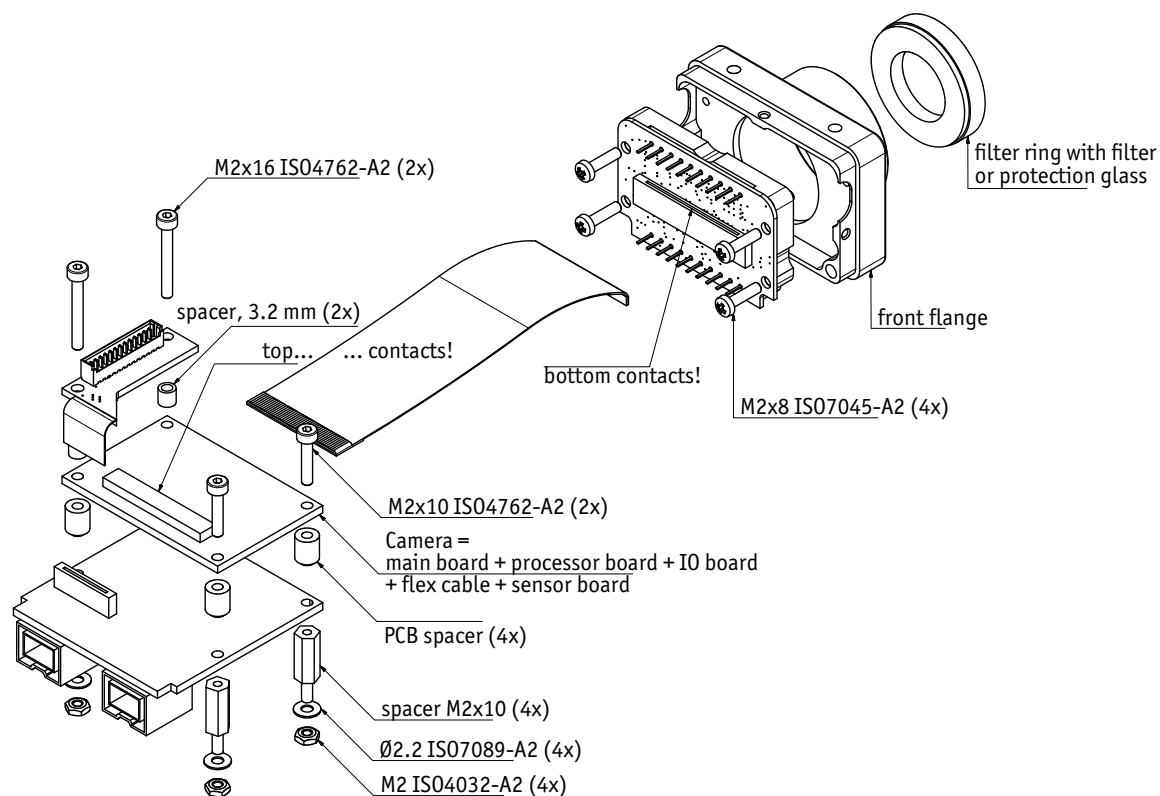
Figure 36: Stingray board level: C-Mount
