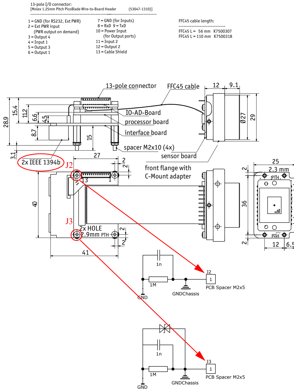
Figure 39: Board level camera: two IEEE 1394b FireWire connectors
