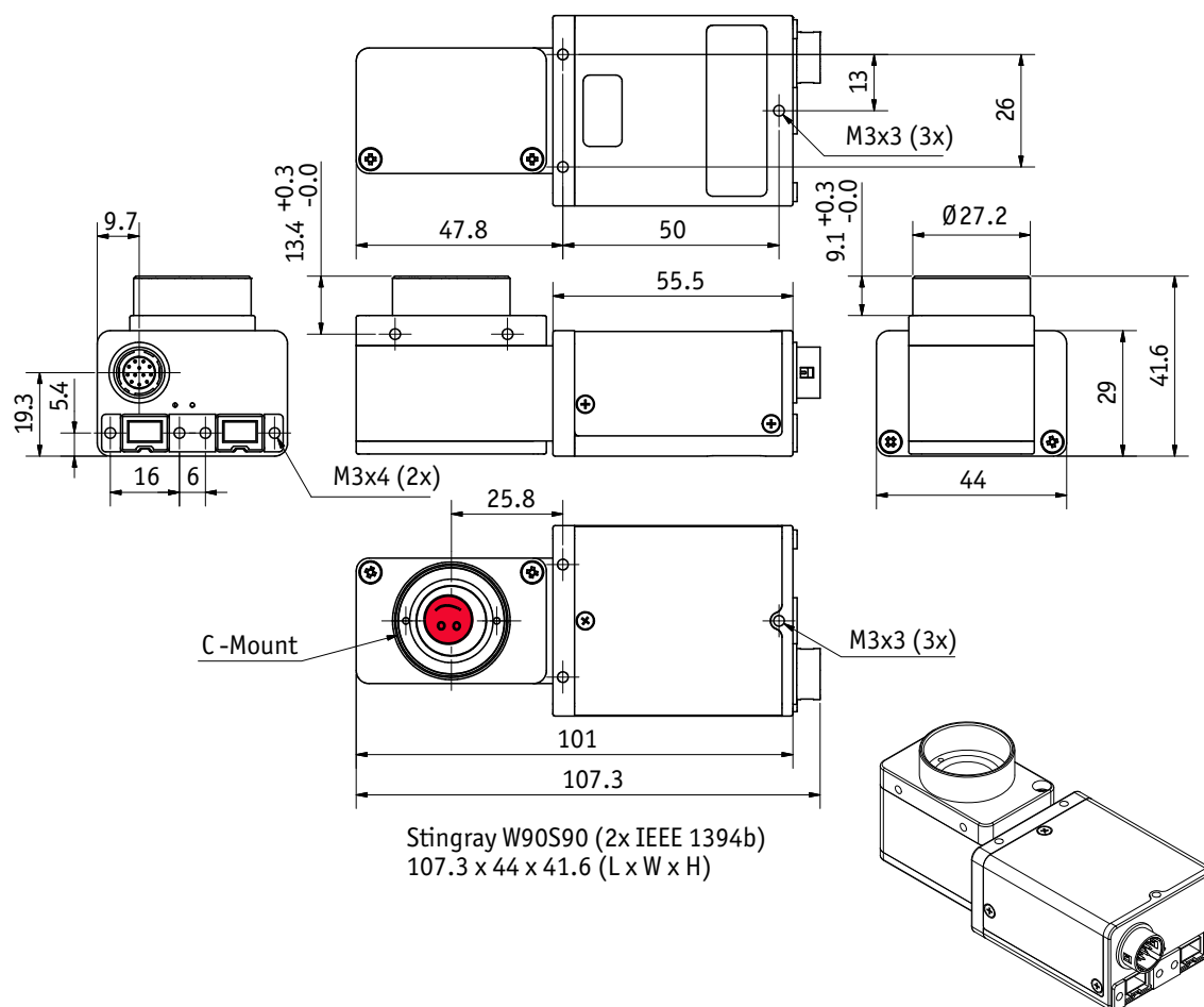
Figure 26: Stingray W90 S90 (2 x IEEE 1394b copper)
