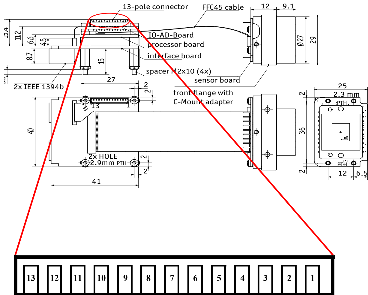
Figure 41: Board level camera: I/O pin assignment
