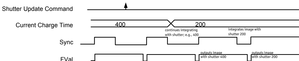
Figure 82: Former standard timing
