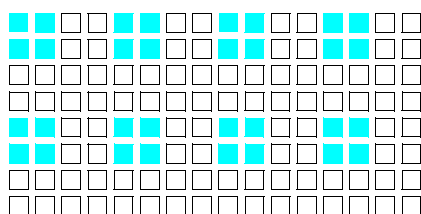
Figure 77: 2 out of 4 H+V sub-sampling (monochrome)
