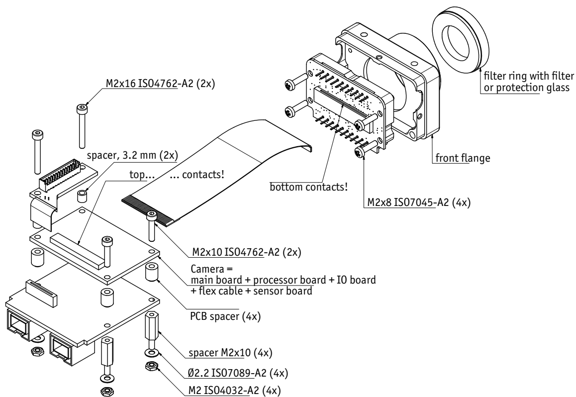
Figure 35: Stingray board level: CS-Mount
