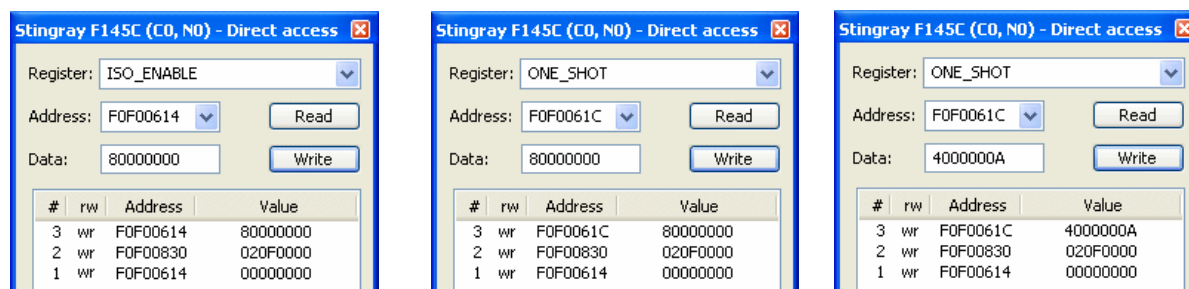
Figure 90: Using Trigger_Mode_15: continuous, one-shot, multi-shot
