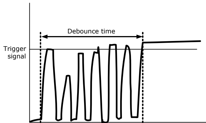
Figure 91: Example of debounce time for trigger
