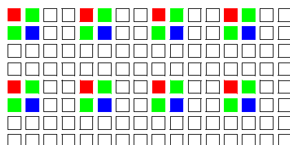
Figure 79: 2 out of 4 H+V sub-sampling (color)
