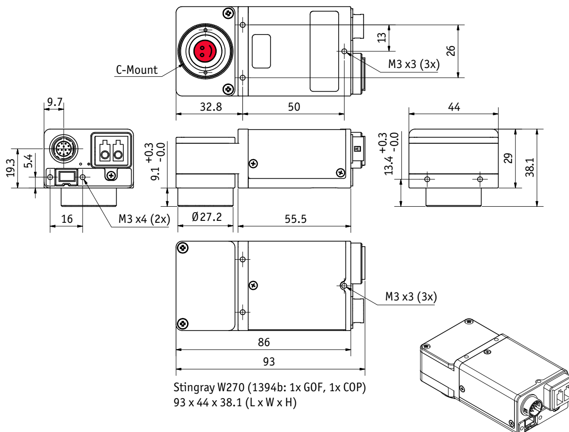
Figure 29: Stingray W270 (IEEE 1394b: 1 x GOF, 1 x copper)
