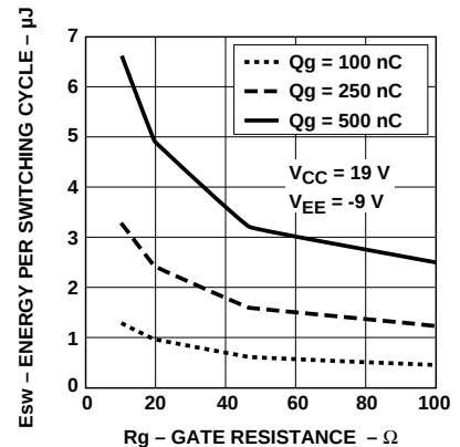
Figure 27. Energy Dissipated in the HCPL-3150 for Each IGBT Switching Cycle.
