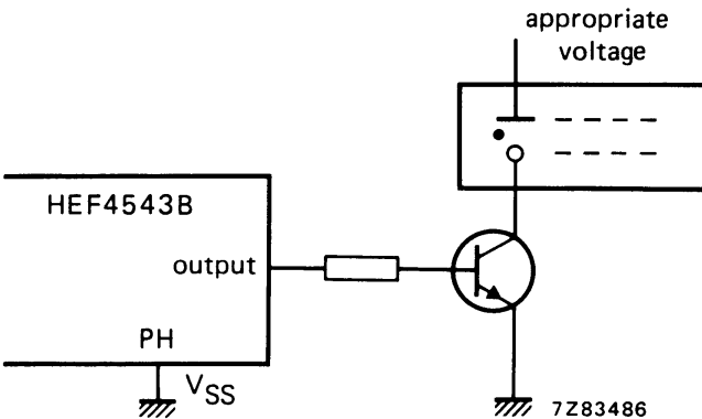
Fig.10 Connection to gas discharge display readout.
