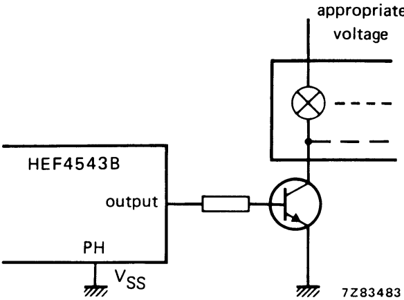
Fig.9 Connection to incandescent display readout.
