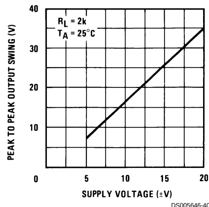
Voltage Swing
