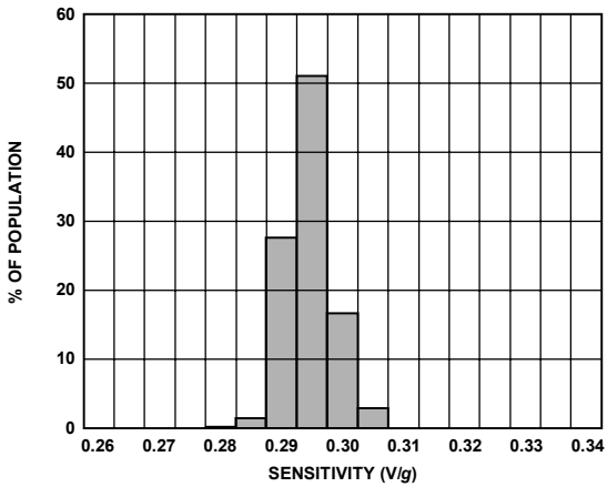
Figure 17. X-Axis Sensitivity at 25°C, V_s = 3 V
