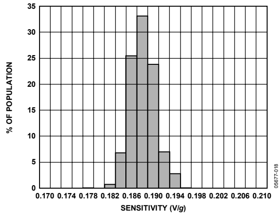
Figure 20. X-Axis Sensitivity at 25°C, V_s = 2 V
