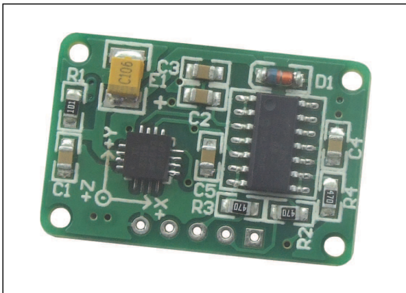
Figure 1: Accel Board
