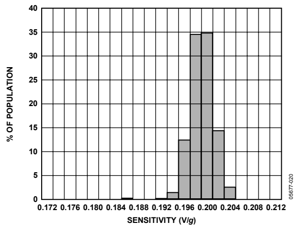
Figure 22. Z-Axis Sensitivity at 25°C, V_s = 2 V
