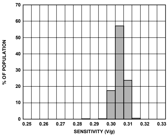
Figure 19. Z-Axis Sensitivity at 25°C, V_s = 3 V
