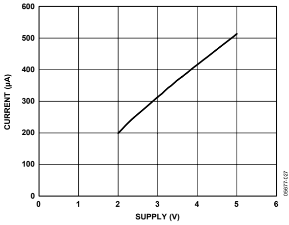
Figure 29. Typical Current Consumption vs. Supply Voltage
