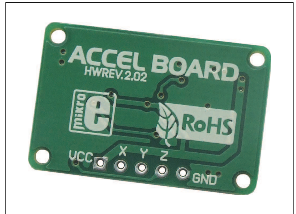
Figure 2: Back side of the Accel Board
