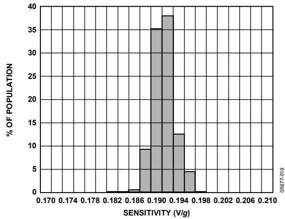
Figure 21. Y-Axis Sensitivity at 25°C, V_s = 2 V
