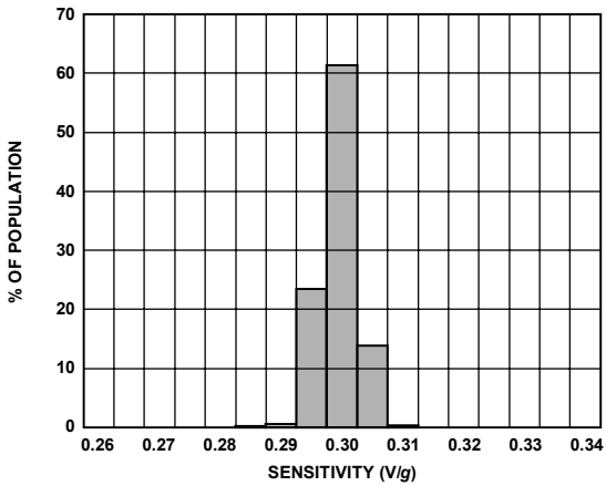
Figure 18. Y-Axis Sensitivity at 25°C, V_s = 3 V
