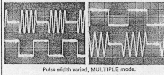
Figure 3-11. Burst Operation.
