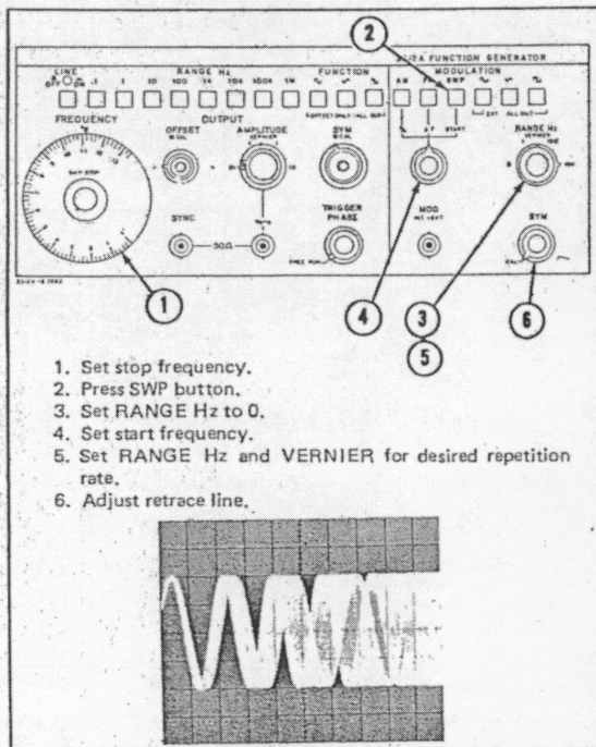
Figure 3-10. Sweep Operation.
