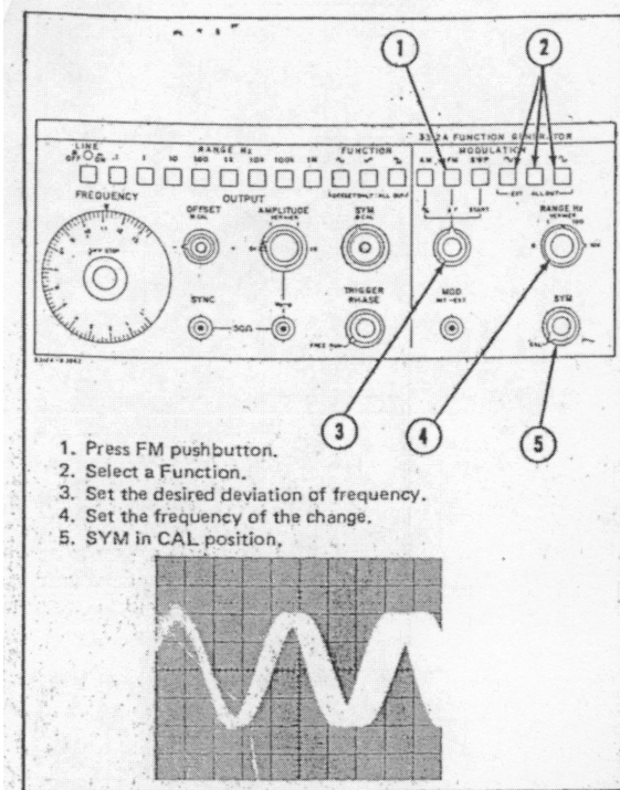
Figure 3-9. FM Operation.
