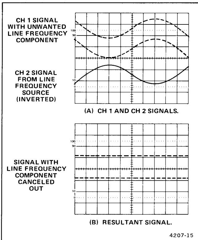
Figure 4-5. Common-mode rejection.
