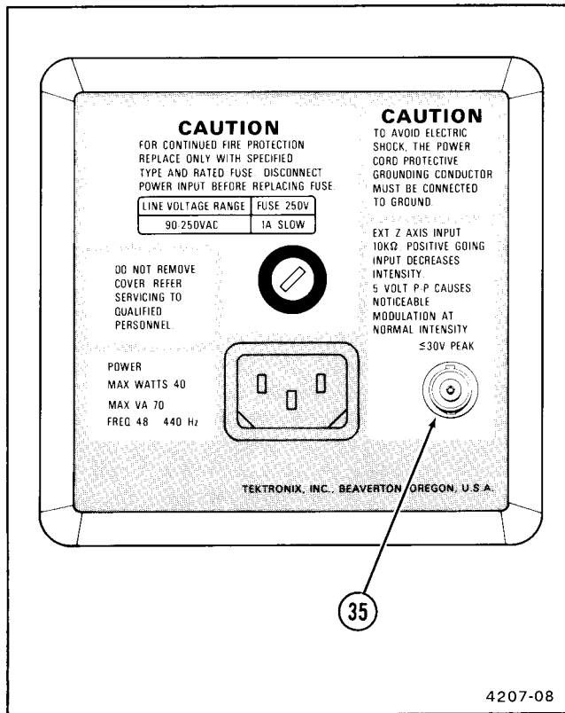
Figure 2-7. Rear-panel connector.
