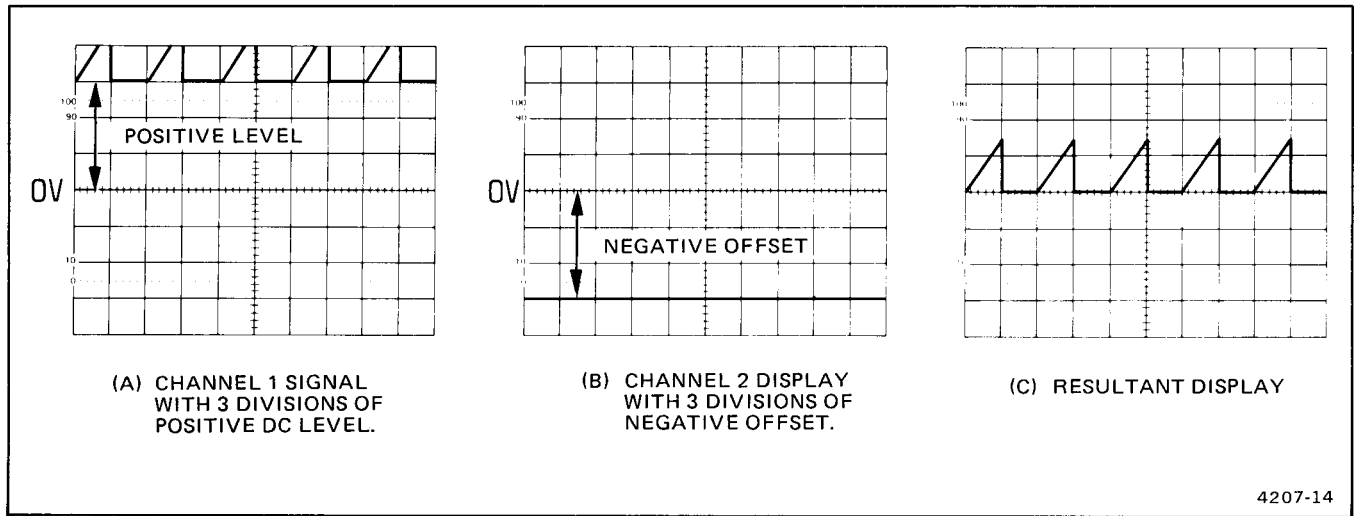
Figure 4-4. Algebraic addition.
