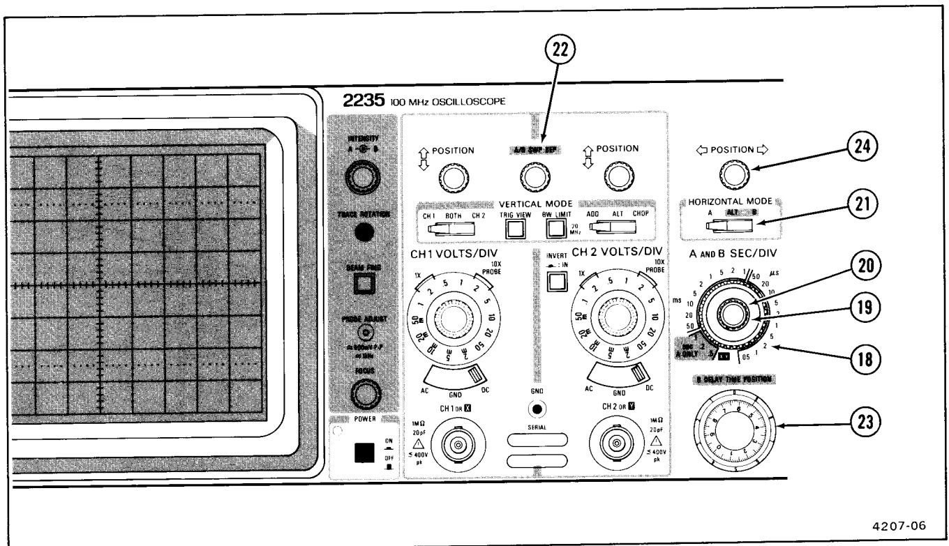
Figure 2-5. Horizontal controls.
