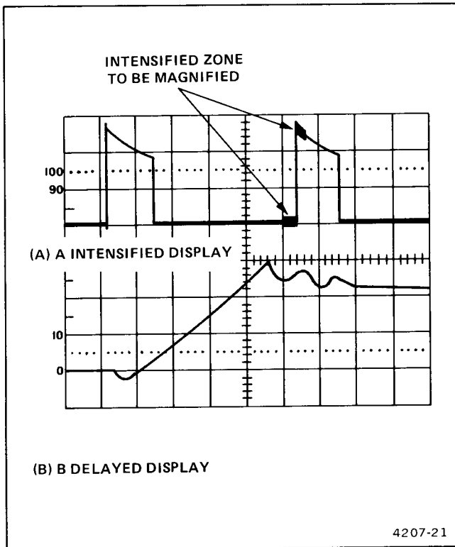
Figure 4-11. Delayed-sweep magnification.
